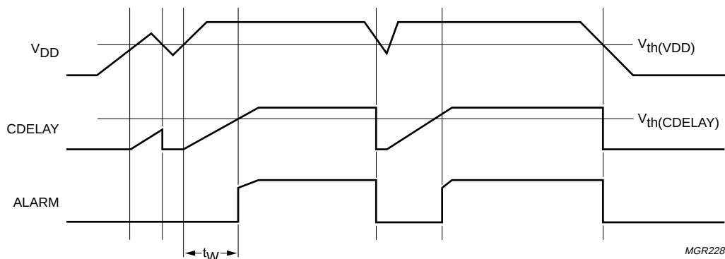
Fig.4 Voltage supervisor.
