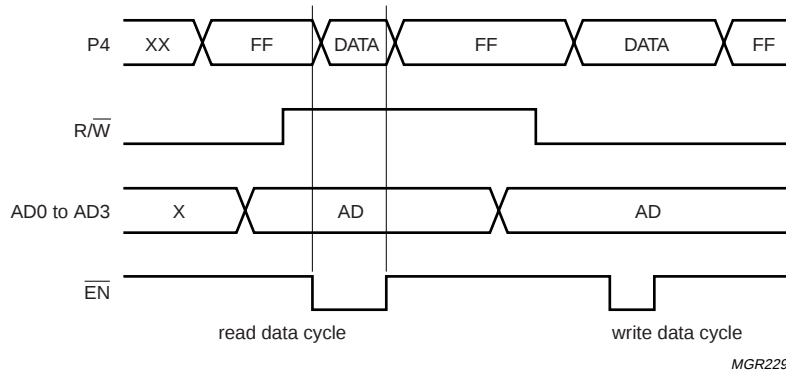
Fig.5 Use of peripheral interface.
