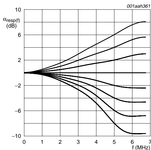
Fig 10. Video equalizer curves
