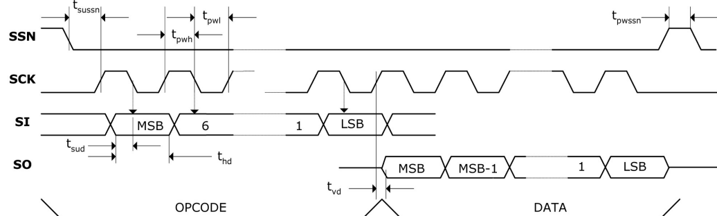
Figure 2-2: SPI Read
