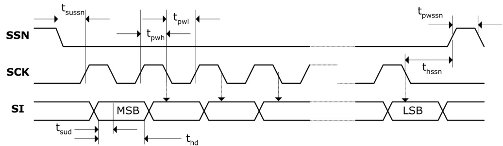
Figure 2-1: SPI Write
