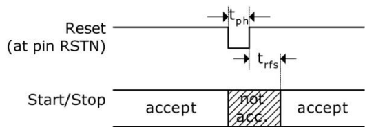
Figure 2-5 Reset Timings
