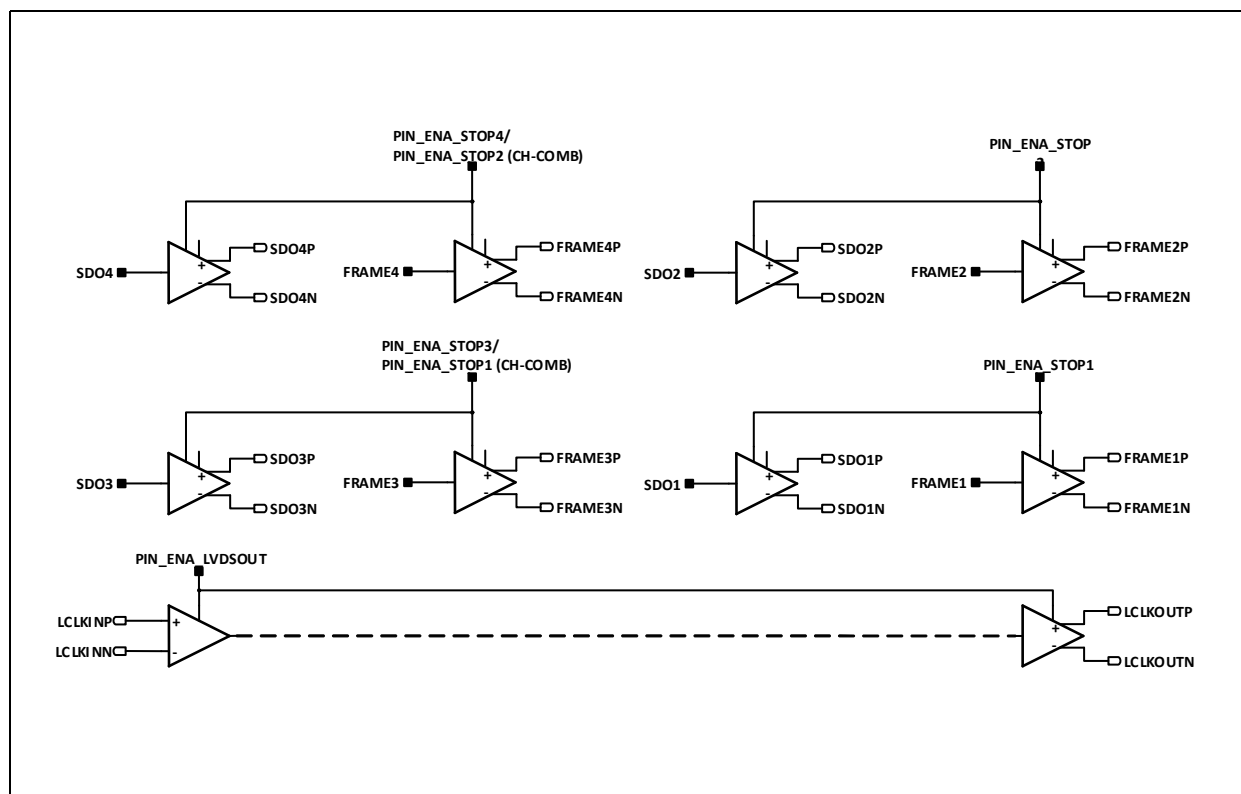
Figure 43: LVDS Outputs
