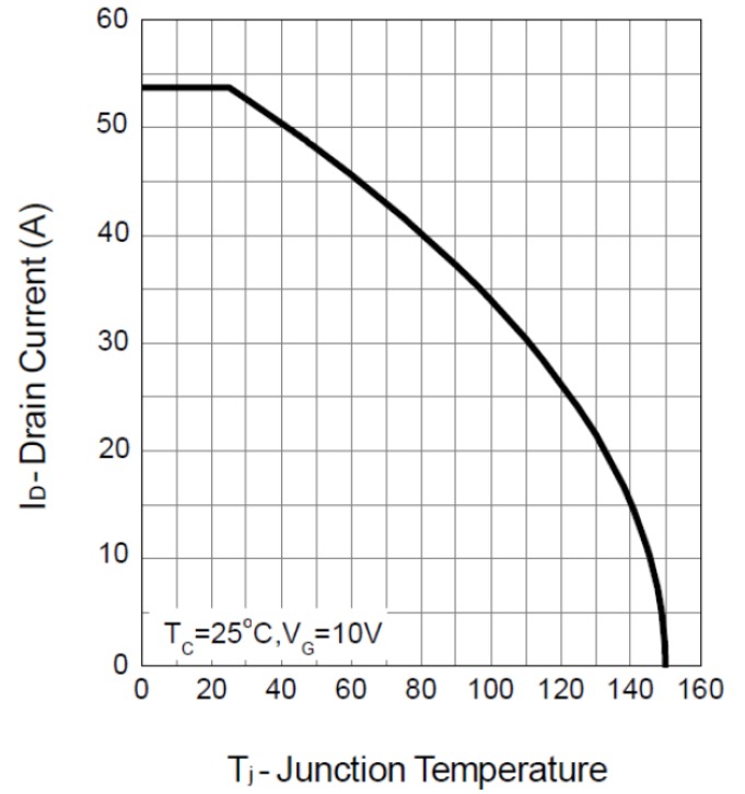
Drain Current
