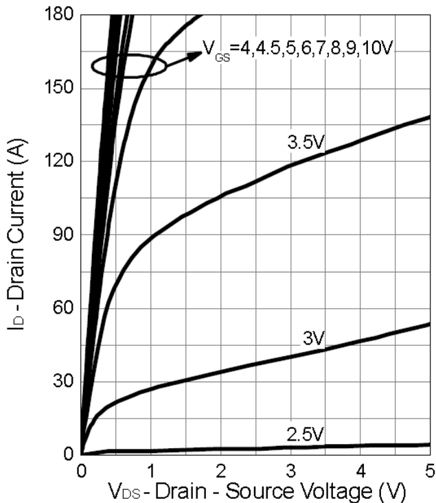
Output Characteristics
