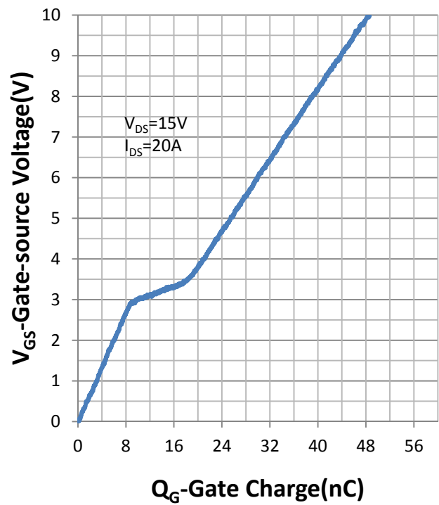
Gate Charge
