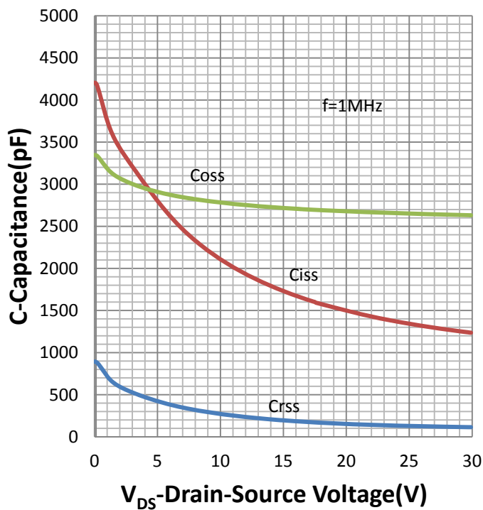
Capacitance
