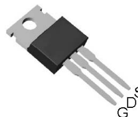
Top View of TO-220
