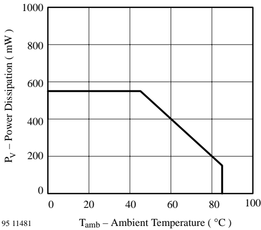
95 11481 T_{amb} – Ambient Temperature ( ^{\circ}C ) Figure 1. Power Dissipation vs. Ambient Temperature
