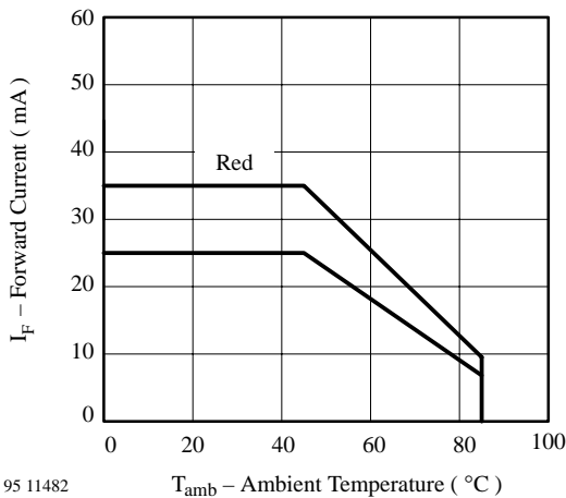
95 11482 T_{amb} – Ambient Temperature ( ^{\circ}C ) Figure 2. Forward Current vs. Ambient Temperature
