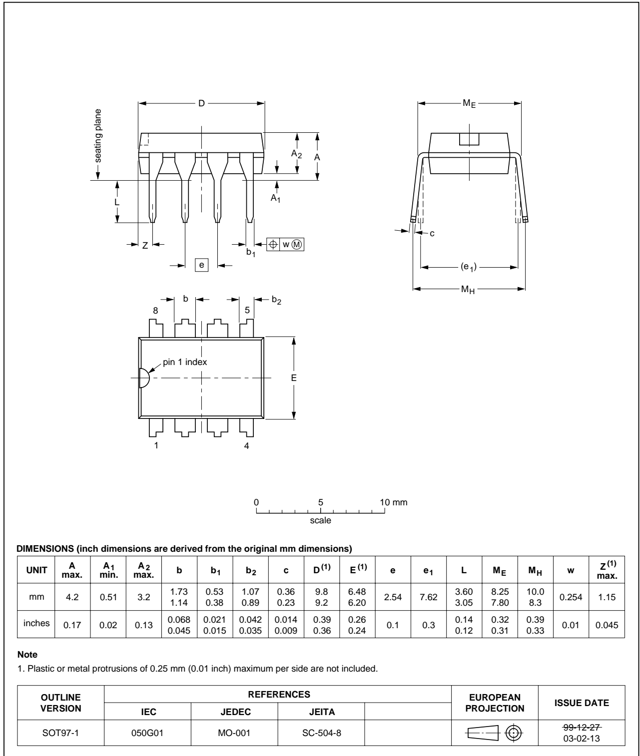
www.DataSheet4U.com Fig 6. Package outline.
