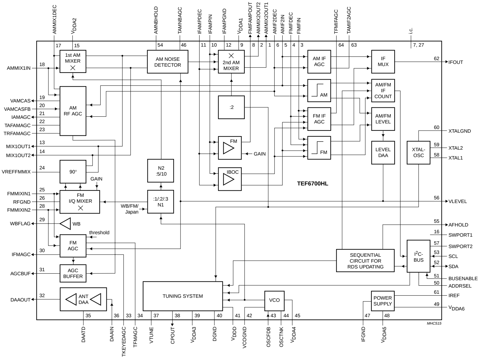
Fig.1 Block diagram.
