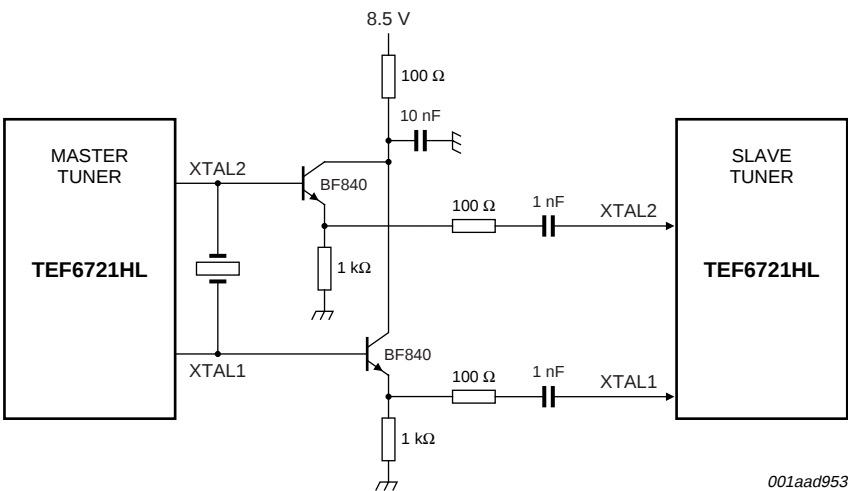
Fig 10. Driving two tuners with one crystal
