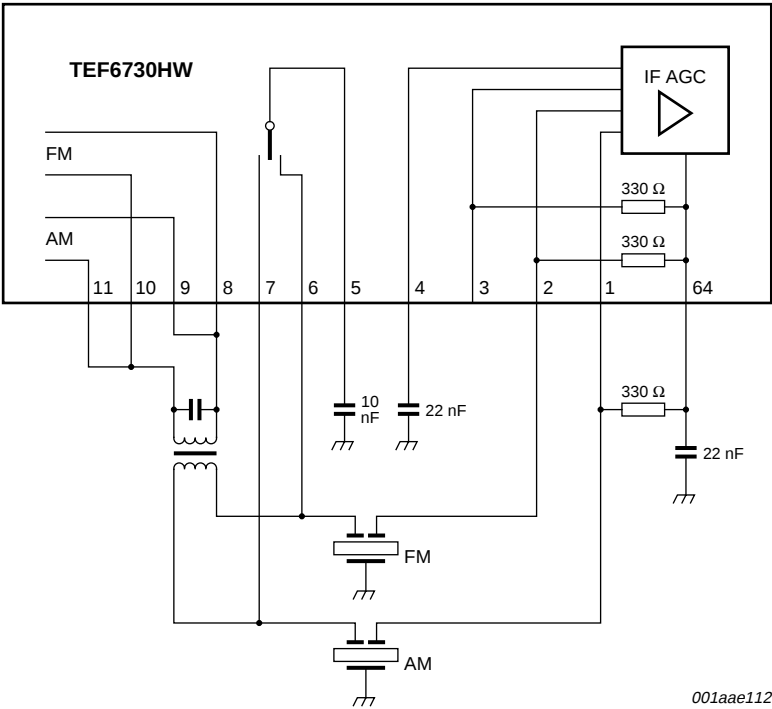
Fig 29. FM and AM (narrow band) mode
