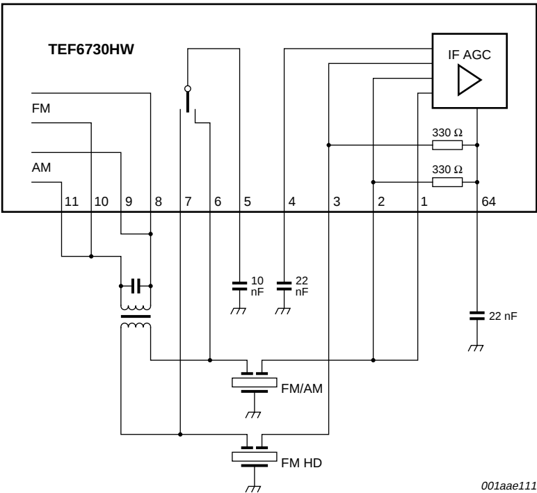
Fig 28. FM/AM and FM HD mode
