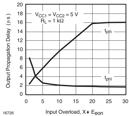
Fig. 7 Propagation Delay vs. Input Overload
