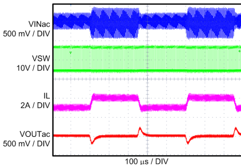
Figure 4. Transient Load Response
