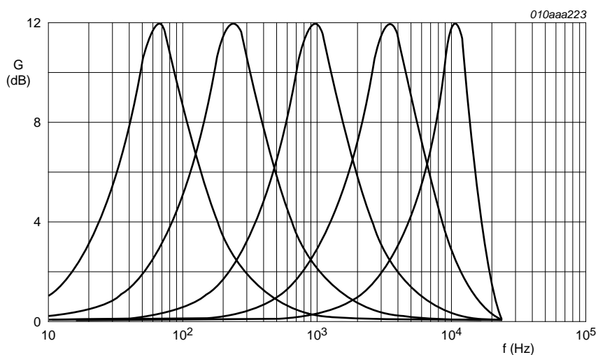
Fig 8. Transfer functions for selected values of f_c , the center frequency
