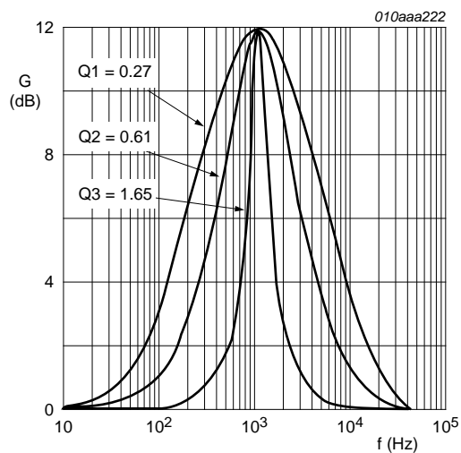
Fig 7. Transfer functions for selected values of Q , the quality factor
