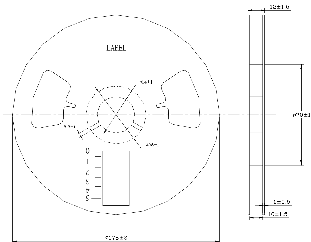
Figure 3 Dimensions of Paper Reel
