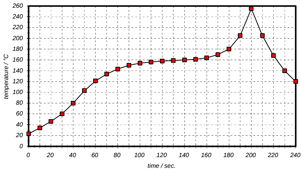
Air reflow profile
