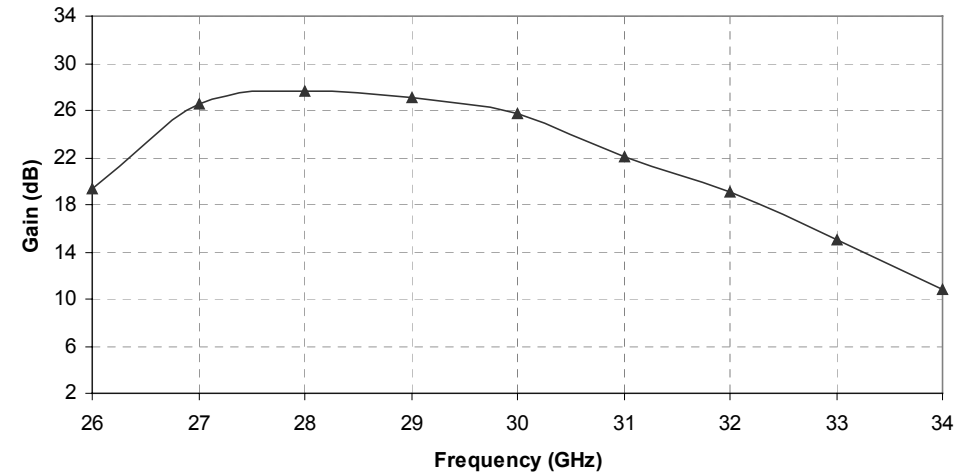
TGA1073B Average Performance Sample Size = 11499 devices
