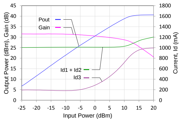
Pout, Gain, Id vs. Pin @ 7.5 GHz
