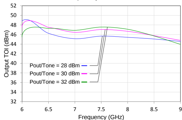
TOI vs. Frequency vs. Pout/Tone
