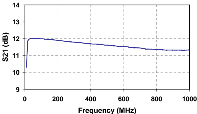
TGA2801B Gain
