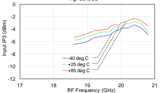
Input IP3 vs. Frequency vs. Temperature
