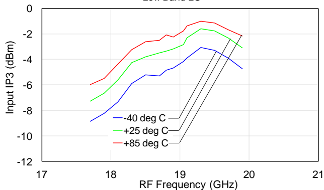
Input IP3 vs. Frequency vs. Temperature
