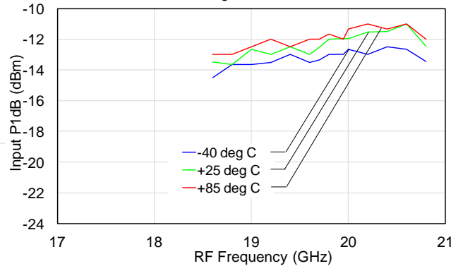
Input P1dB vs. Frequency vs. Temperature
