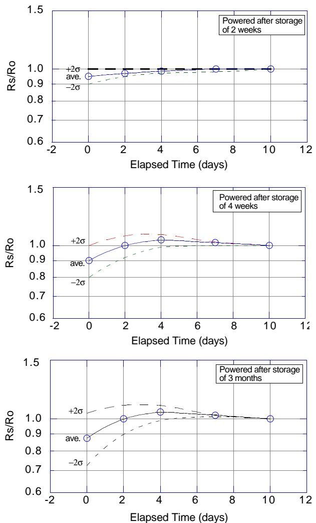
Figure 13 - Time dependency ( R_o = 1.0 ) (20 samples tested)
