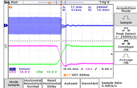
Switching Speed - Off < 18 ns Vc = 0/-20 V, Freq = 500 mHz, Pin = 4dBm, +25 °C
