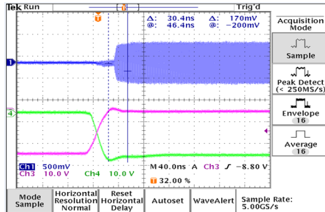
Switching Speed - On < 31 ns Vc = 0/-20 V, Freq = 500 mHz, Pin = 4dBm, +25 °C
