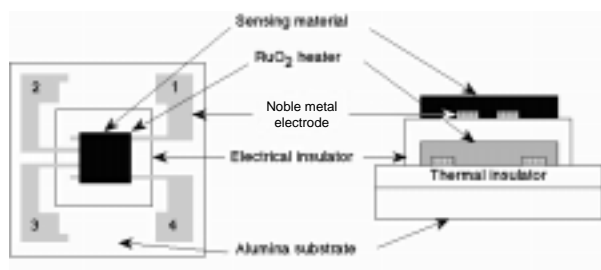
Figure 1 - Sensor structure
