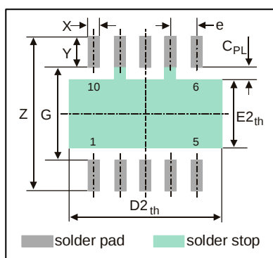
Fig. 8: PCB land pattern style
