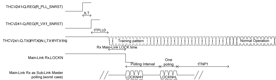
Figure 22. Lock Sequence
