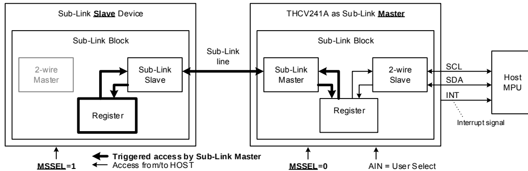
Figure 16. Host MPU to Sub-Link Slave Register via THCV241A access configuration
