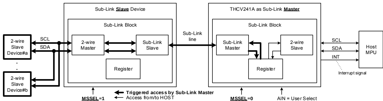
Figure 17. Host MPU to 2-wire slave devices connected to Sub-Link Slave via THCV241A access configuration
