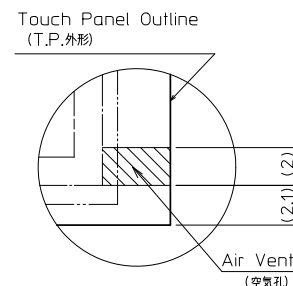
DETAIL C(5:1)
