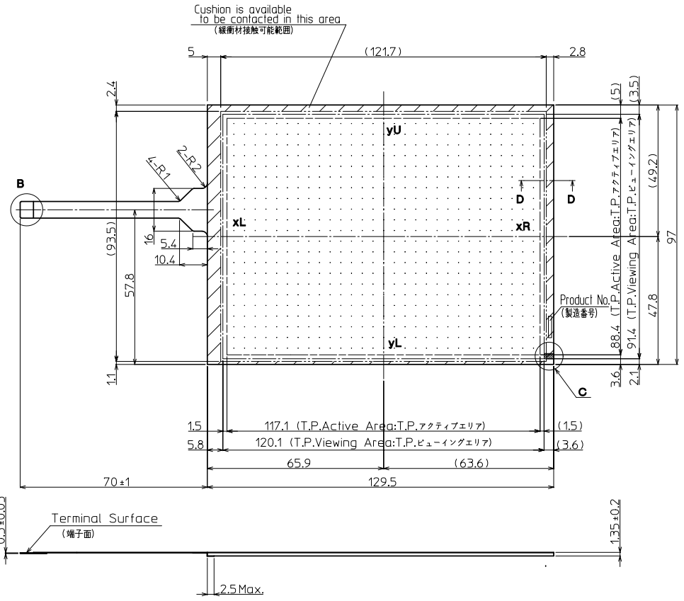
Touch Panel Outline (T.P.外形)
