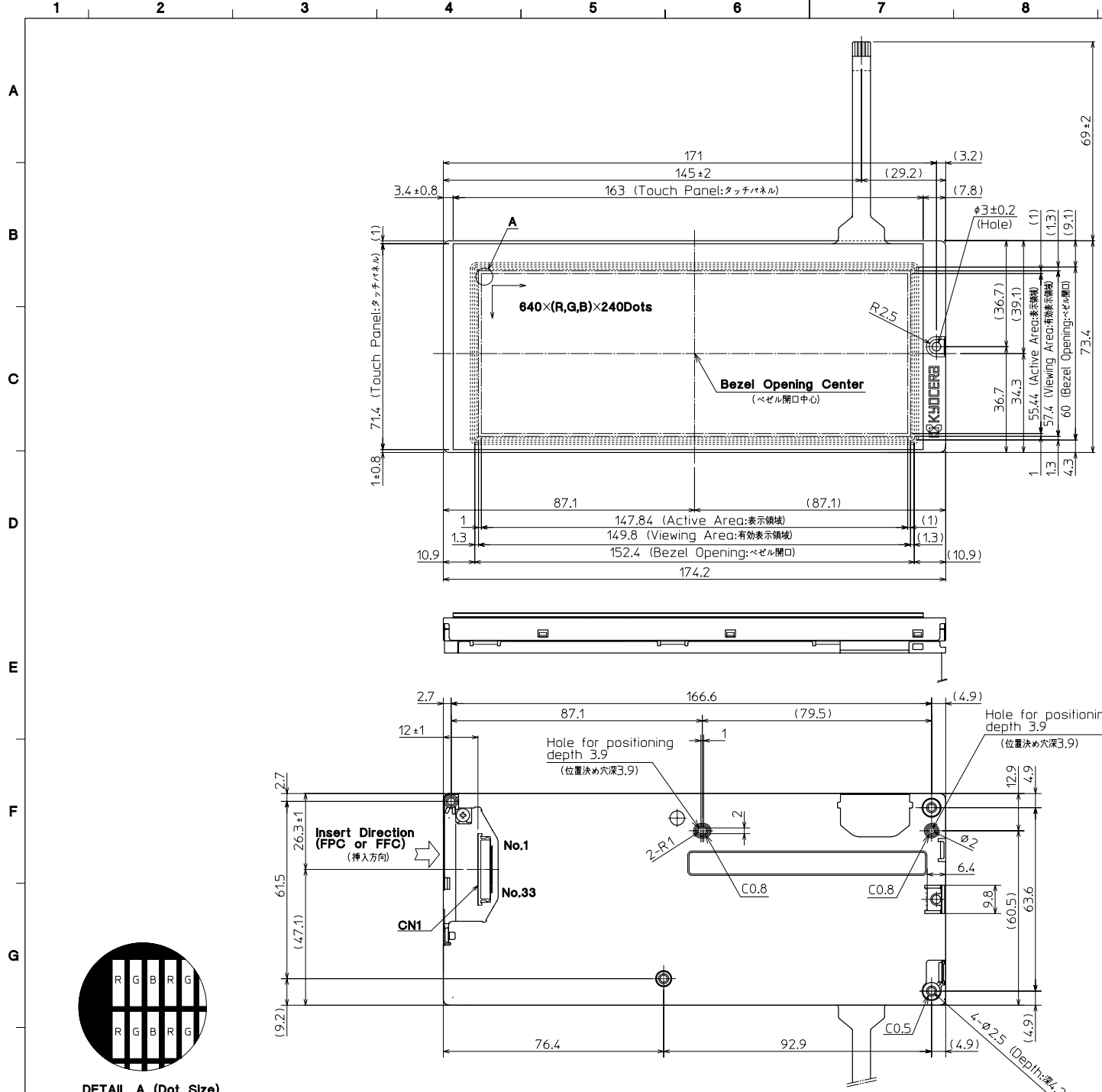
DETAIL A (Dot Size) (NTS)
