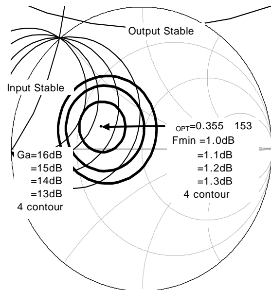
Noise Figure Contours & Constant Gain f = 1\text{GHz}, V_{CE} = 8V, I_{cc} = 5\text{mA}
