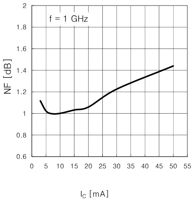
NF vs. I C V CE = 3 V, I C = parameter, Z S = Z Sopt
