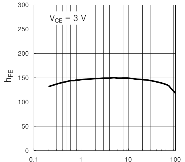
h_{FE} vs. I_C
