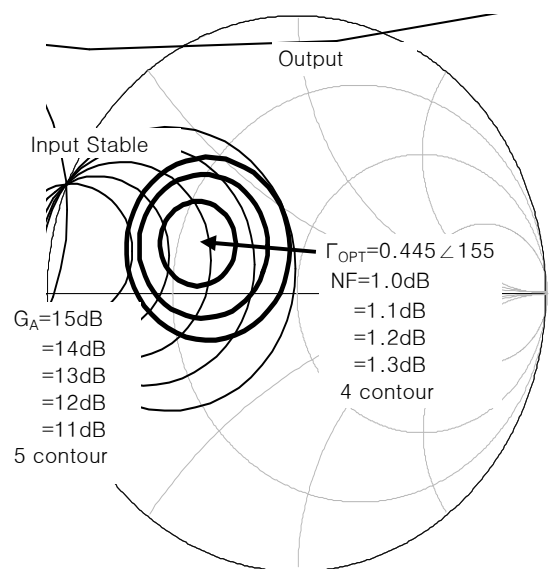
Noise Figure Contours & Constant Gain f = 1 GHz, V CE = 3 V, I C = 7 mA
