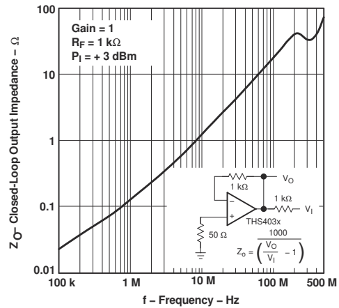
Figure 5-41. Closed-loop Output Impedance vs Frequency
