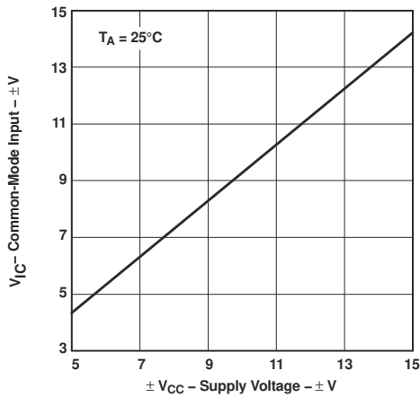
Figure 5-40. Common-mode Input Voltage vs Supply Voltage
