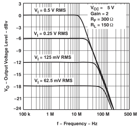
Figure 5-66. Output Amplitude vs Frequency
