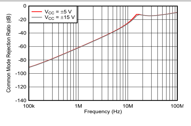
Figure 5-12. Common-mode Rejection Ratio vs Frequency
