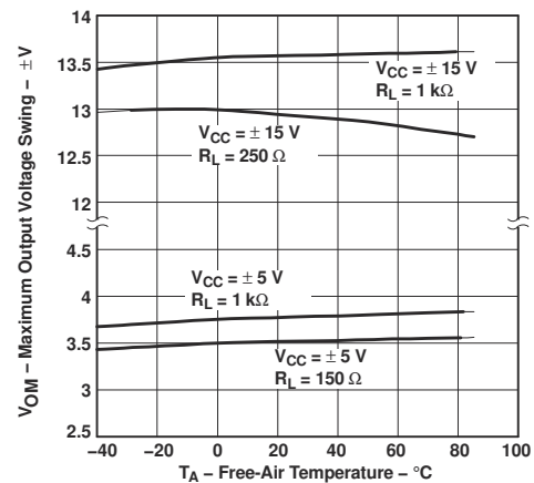
Figure 5-37. Maximum Output Voltage Swing vs Free-air Temperature
