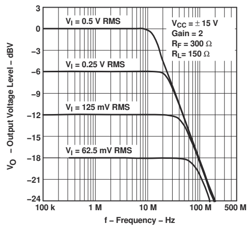
Figure 5-65. Output Amplitude vs Frequency
