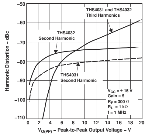
Figure 5-48. Harmonic Distortion vs Peak-to-peak Output Voltage
