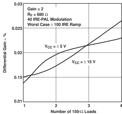
Figure 5-72. Differential Gain vs Number of 150- \Omega Loads
