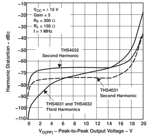
Figure 5-49. Harmonic Distortion vs Peak-to-peak Output Voltage
