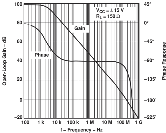
Figure 5-42. Open-loop Gain and Phase Response
