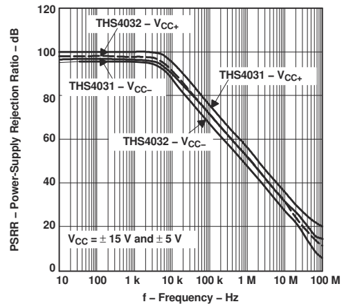
Figure 5-43. Power-supply Rejection Ratio vs Frequency
