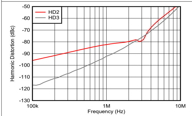
Figure 5-15. Harmonic Distortion vs Frequency
