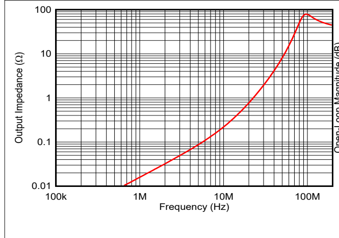
Figure 5-9. Closed-Loop Output Impedance
