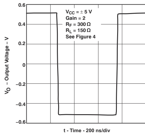
Figure 5-73. 1-V Step Response
