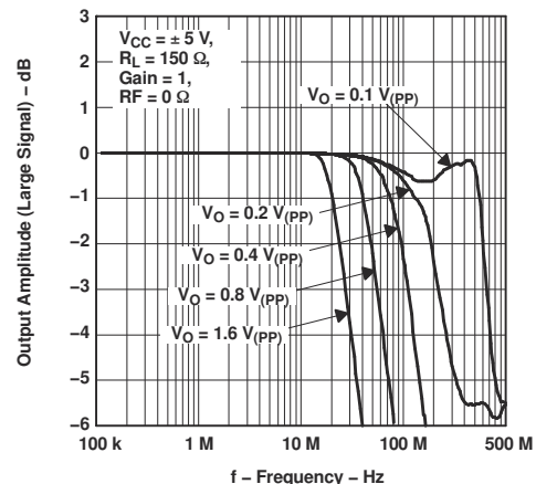
Figure 5-59. Frequency Response With Varying Output Voltage Swing
