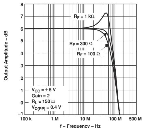
Figure 5-61. Small-signal Frequency Response With Varying Feedback Resistance
