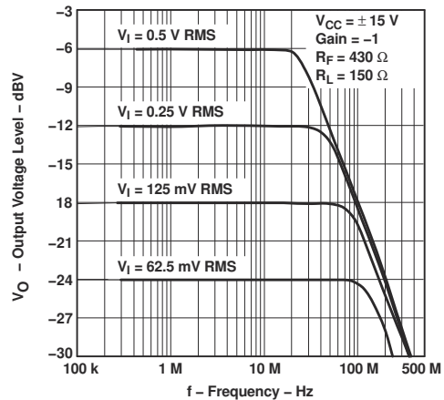
Figure 5-67. Output Amplitude vs Frequency
