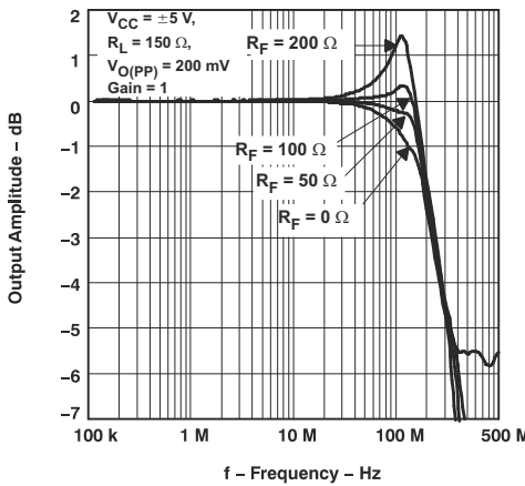
Figure 5-58. Small Signal Frequency Response With Varying Feedback Resistance
