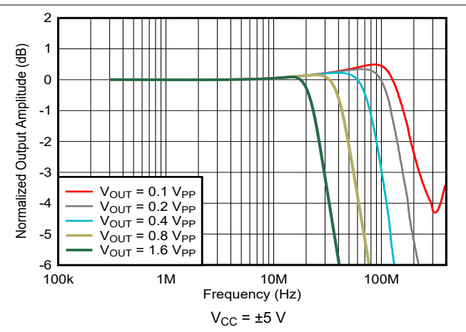
Figure 5-8. Large-Signal Frequency Response
