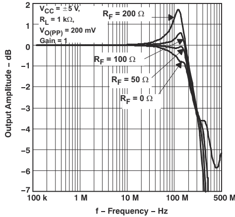
Figure 5-56. Small Signal Frequency Response With Varying Feedback Resistance
