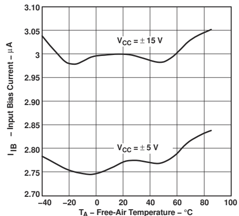
Figure 5-35. Input Bias Current vs Free-air Temperature
