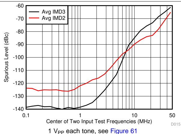
Figure 15. IMD2 and IM3 Over Frequency
