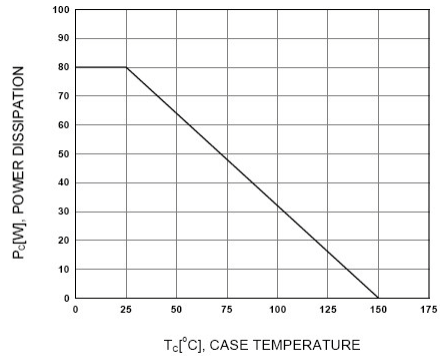
Figure 6. Power Derating
