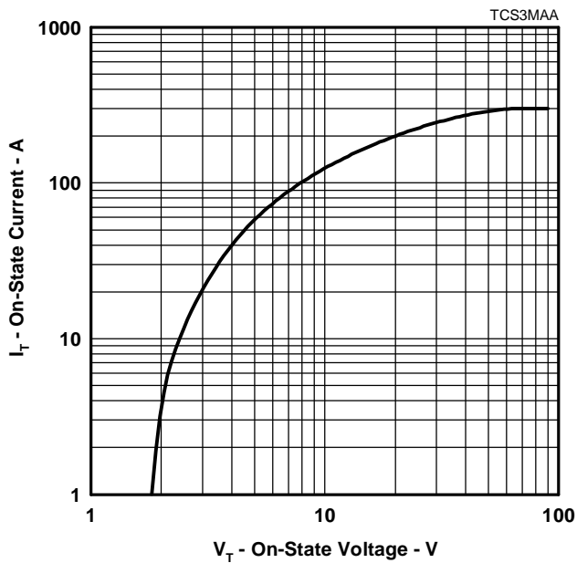
ON-STATE CURRENT vs ON-STATE VOLTAGE
