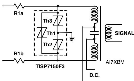
Figure 37. ISDN PROTECTION
