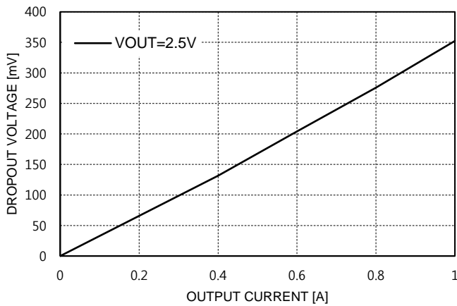
Dropout Voltage
