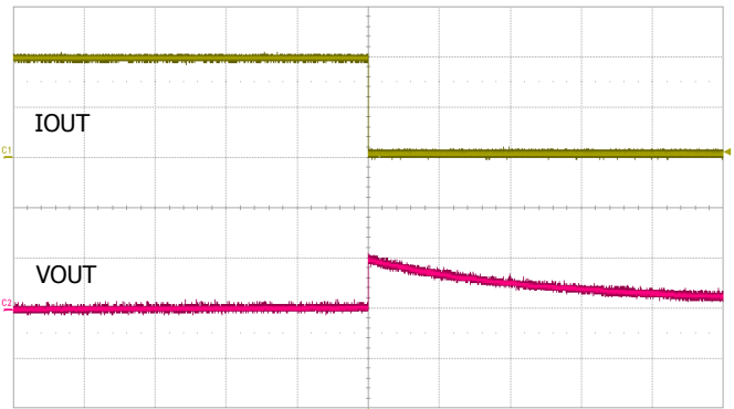
(IOUT: 500mA/div, VOUT: 50mV/div, Time: 10ms/div)
