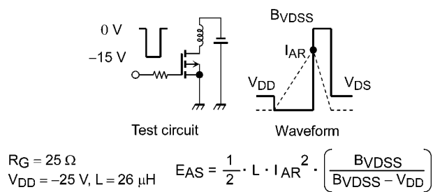
Fig. 9.15 Test Circuit/Waveform
