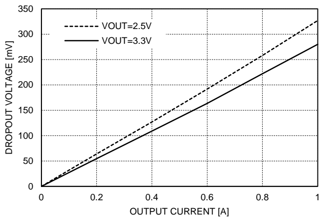
Dropout Voltage
