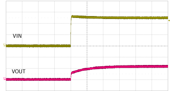
VOUT = 1.2V ( C ss = 220pF, C f = 1 \mu F )
