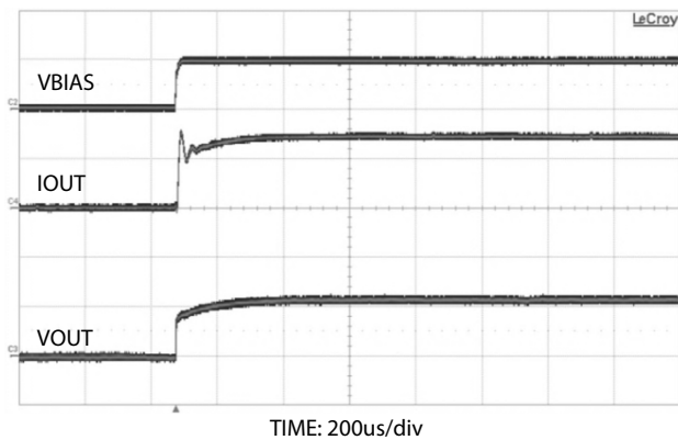
V_{BIAS} & V_{IN} Start Up Transient Response
