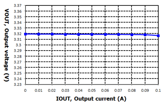
IOUT vs. VOUT
