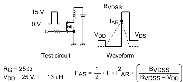
Fig. 9.15 Test Circuit/Waveform
