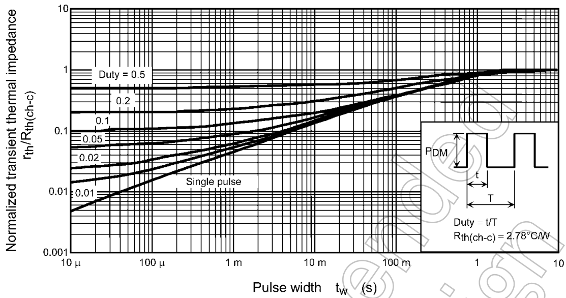
Fig. 8.13 r_{th}/R_{th}(ch-c) - t_w (Guaranteed Maximum)
