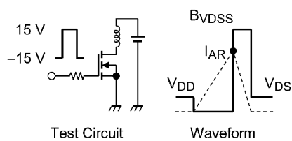
Fig. 8.16 Test Circuit/Waveform
