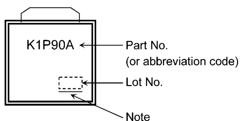
Fig. 7.1 Marking
