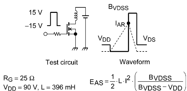
Fig. 8.16 Test Circuit/Waveform
