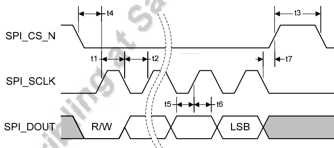
Figure 31. SPI Write Timing
