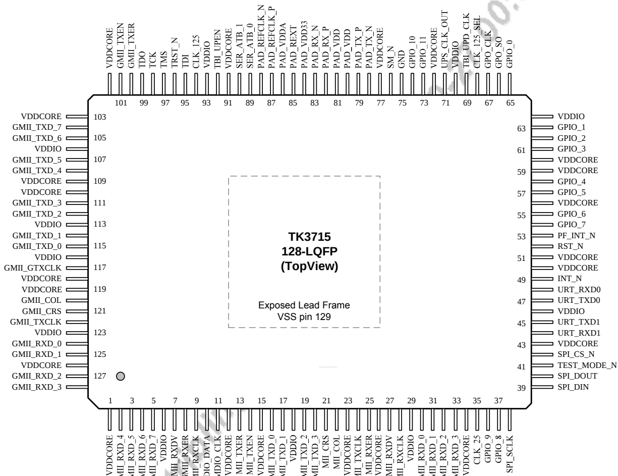
Figure 2. TK3715 Pin Diagram in 128-LQFP Package
