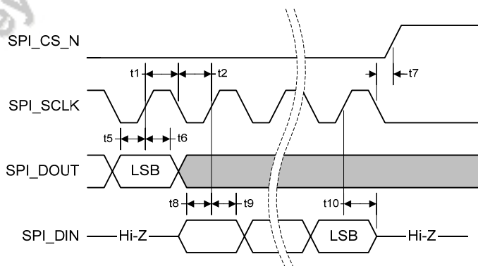
Figure 32. SPI Read Timing
