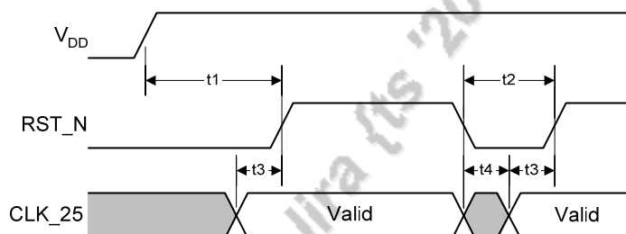
Figure 33. Reset and CLK_25 Timing
