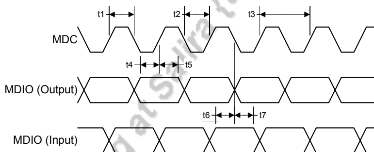
Figure 29. MDIO Timing
