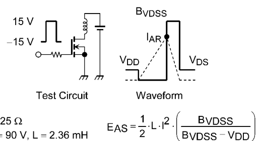
Fig. 8.16 Test Circuit/Waveform
